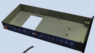
POS enclosure with aperture and fixing points for Display
